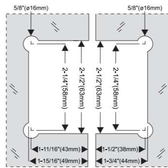
135° Glass-Glass
