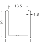
15035-1-CH 1" Shower channel for 12mm Glass
