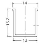
15030 3/4" Shower channel for 10mm Glass
