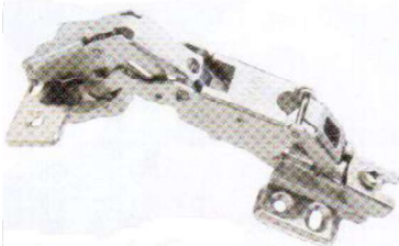
07165A Hinge 4 Hole Plate 165 Degree F/O
