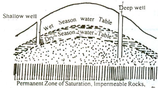
Fig. 5.8 Water Table
