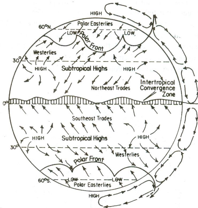
Fig 11.7 : Planetary Winds
