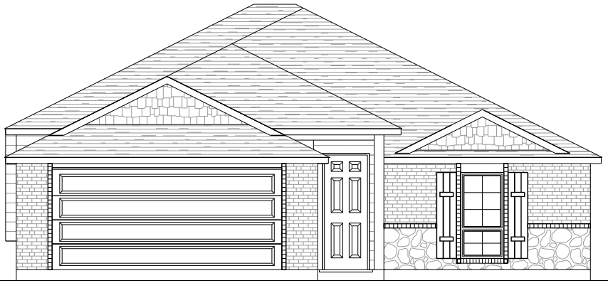
STANDARD ELEVATION
