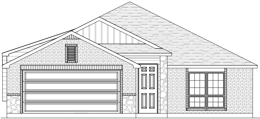
STANDARD ELEVATION
