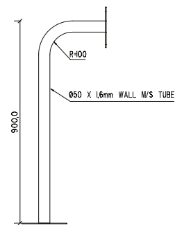
SINGLE GOOSENECK
