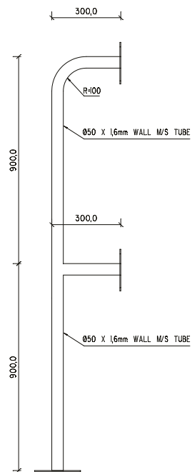
DUAL GOOSENECK
