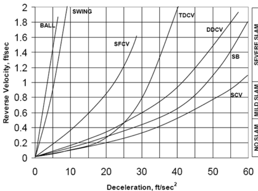
Comparison of Silent Check Valve's(SCV) Dynamic Characteristics
